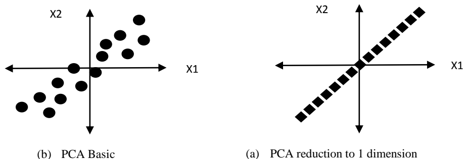
Fig.1.The concept of PCA
